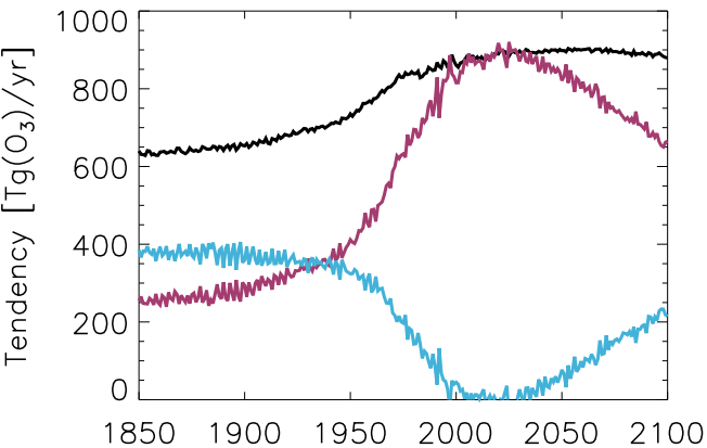
UKESM1-LL-0
