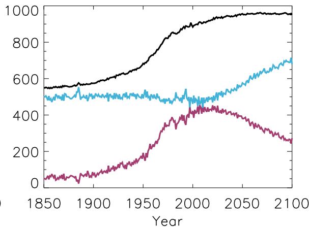
MRI-ESM2-0
