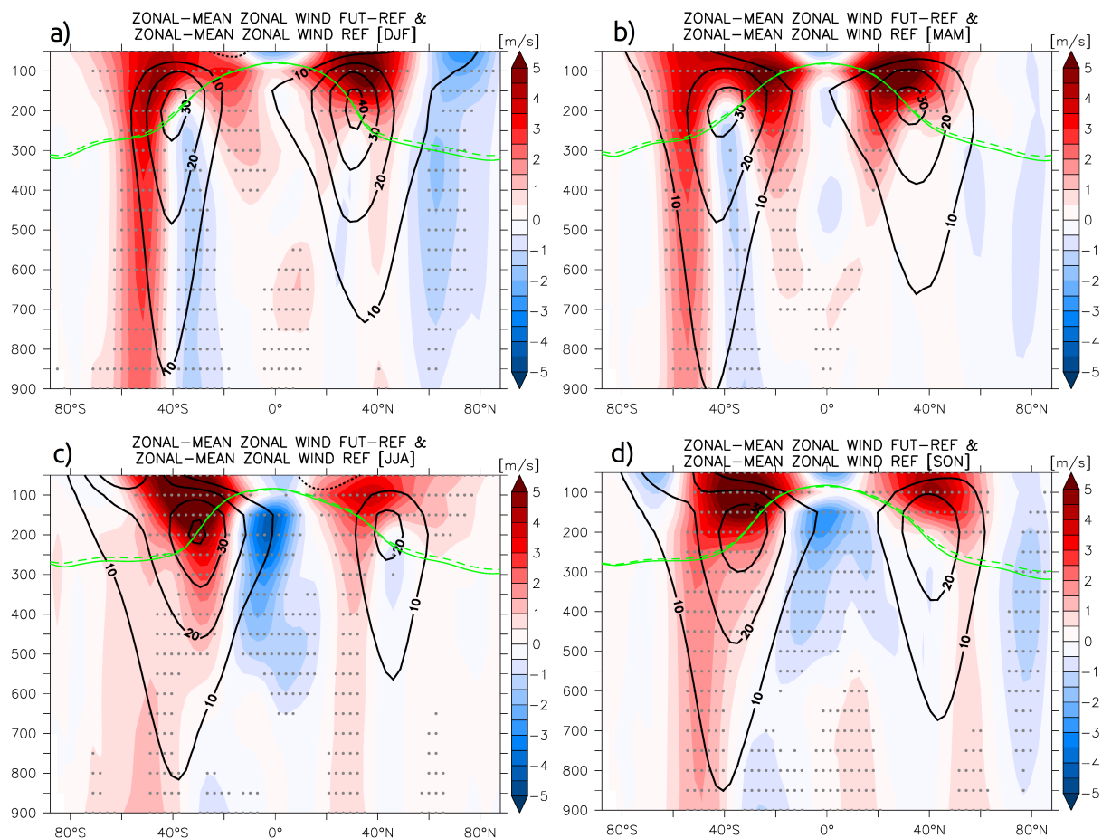
Figure 2. Zonal-mean zonal wind differences ( \text{m s}^{-1} ) between the FUT and REF periods for DJF (a), MAM (b), JJA (c), and SON (d). The black contours indicate the zonal-mean zonal wind climatology ( \text{m s}^{-1} ) for the REF period. The green solid (dashed) line denotes the height of the tropopause during the REF (FUT) period. Grey dots denote statistically significant changes at the 99 % confidence level.
