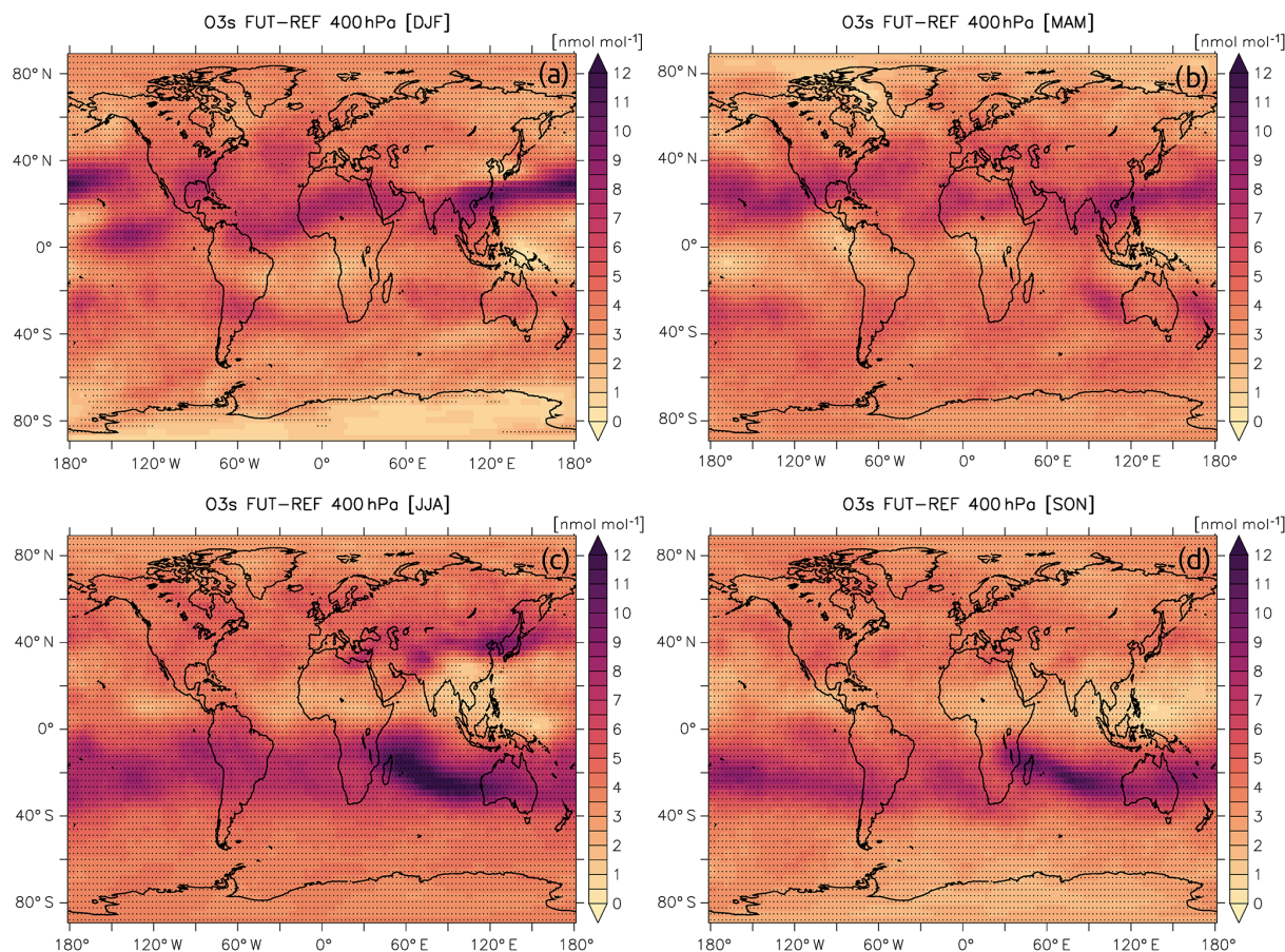
Figure 7. Mean stratospheric ozone tracer ( O_3s ) concentration differences (shaded; \text{nmol mol}^{-1} ) between the FUT and REF periods at 400 hPa for DJF (a), MAM (b), JJA (c), and SON (d). Black dots denote statistically significant differences at the 99 % significance level.
