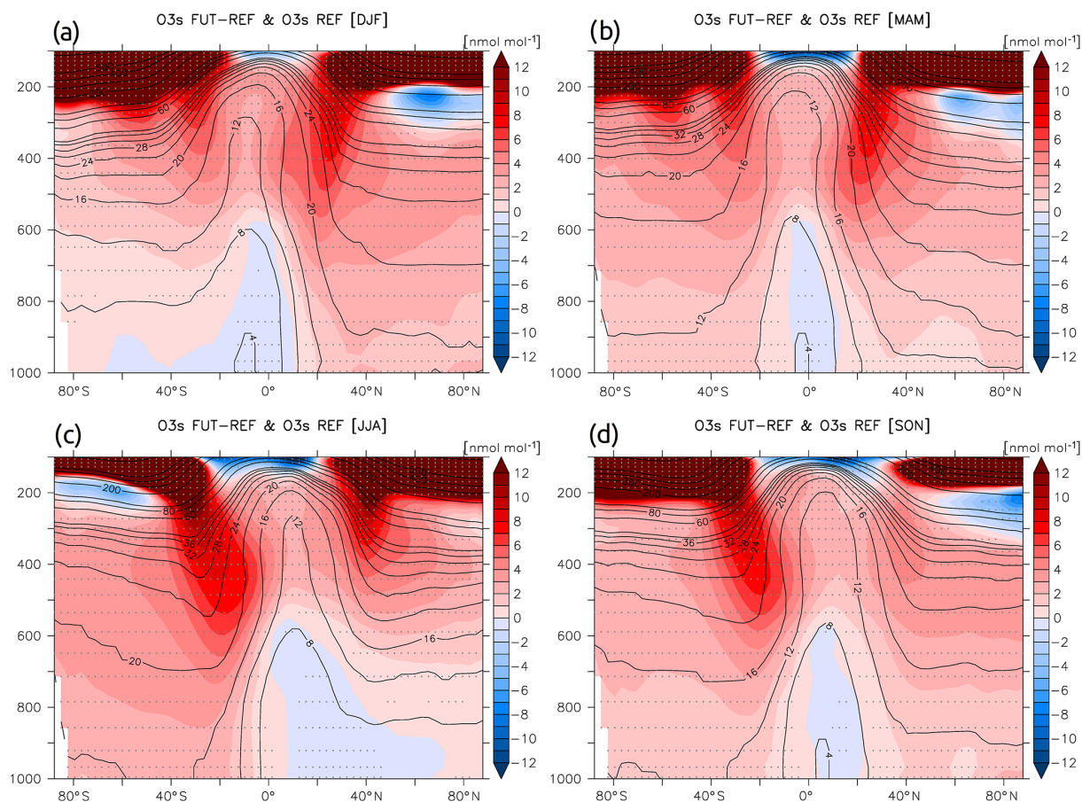
Figure 6. Differences of zonal-mean stratospheric ozone tracer ( \text{O}_3\text{s} ) concentrations between the FUT and REF periods (shaded; \text{nmol mol}^{-1} ) for DJF (a), MAM (b), JJA (c), and SON (d). The black contours denote the zonal-mean stratospheric ozone tracer concentrations ( \text{nmol mol}^{-1} ) during the REF period. Grey dots denote statistically significant changes at the 99% confidence level.
