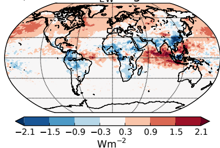
(e) ORG: \Delta AIE_{LW} avg = -0.14 \text{ Wm}^{-2}
