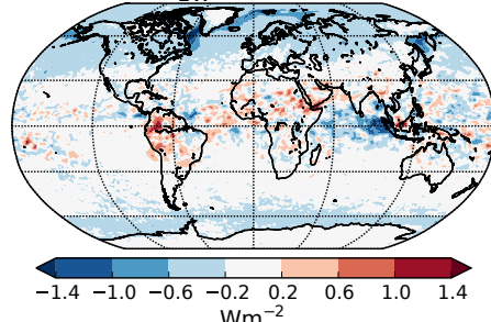
(e) ORG: \Delta AIE_{LW} avg = -0.14 \text{ Wm}^{-2}
