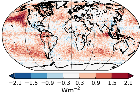
(f) ORG: \Delta AIE_{tot} avg = 0.25 \text{ Wm}^{-2}
