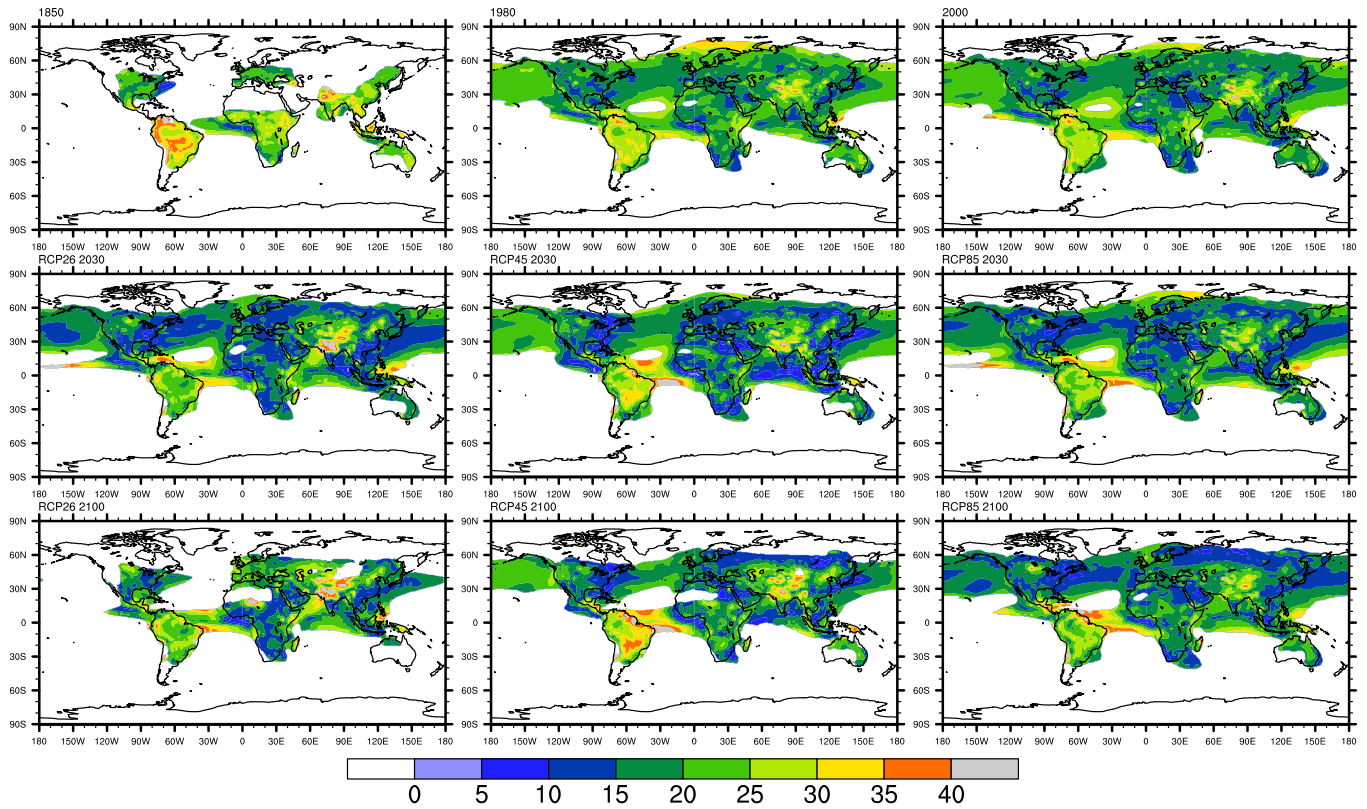
Figure S4. Inter-model standard deviation (in %) of the NO y wet deposition. The standard deviation is only shown for regions where deposition is larger than 50 mg(N)/m 2 /year (see Fig. 5a). The number of models used for each time slice is shown in Table S2.
