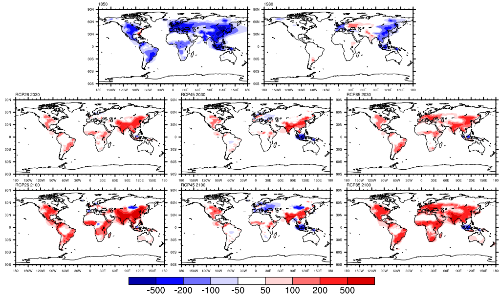
Figure S5b. Total (wet + dry) MMM \text{NX}_x deposition 1850-2100 ( \text{mg(N)m}^{-2}\text{yr}^{-1} ) relative to year 2000. Top row shows 1850 and 1980. Middle row shows 2030 for RCP2.6, RCP4.5 and RCP8.5. Bottom row shows 2100 for RCP2.6, RCP4.5 and RCP8.5.
