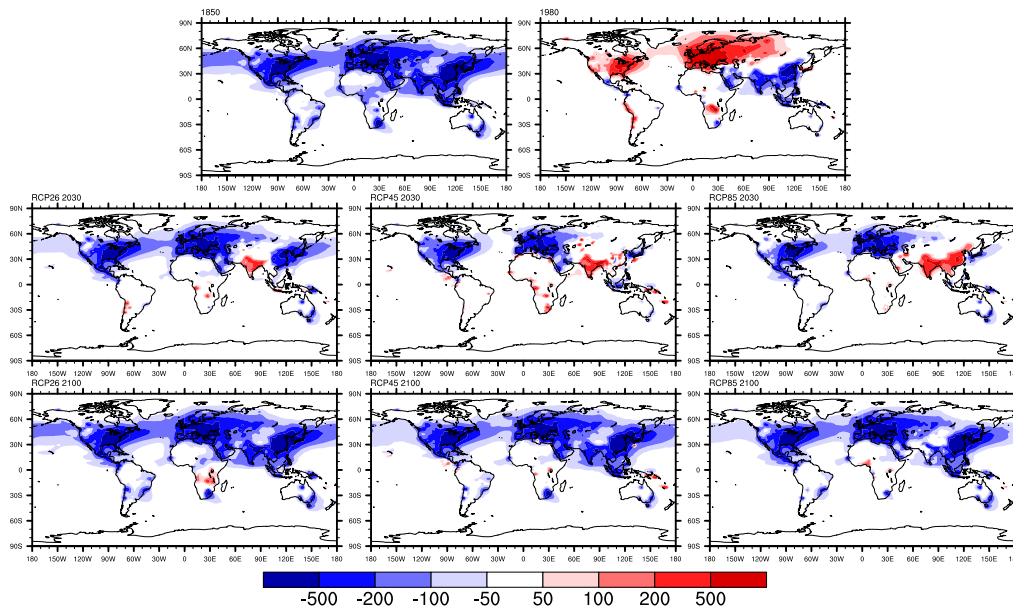
Figure S5c. Total (wet + dry) MMM SO x deposition 1850-2100 (mg(S)m -2 yr -1 ) relative to year 2000. Top row shows 1850 and 1980. Middle row shows 2030 for RCP2.6, RCP4.5 and RCP8.5. Bottom row shows 2100 for RCP2.6, RCP4.5 and RCP8.5.
