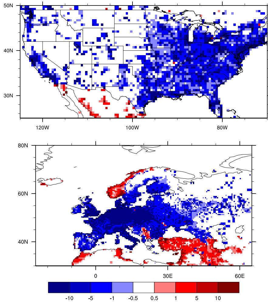
Figure S1c. Change in SO 2 anthropogenic emissions (2000-1980) in 10 -2 mg(S)/m 2 /year.
