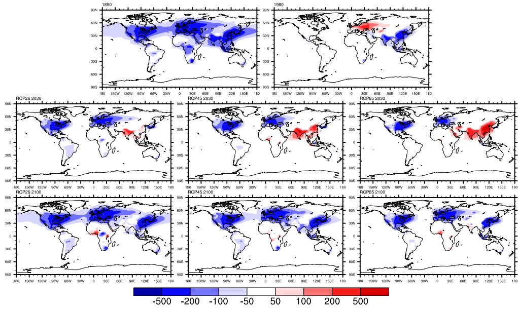
Figure S5a. Total (wet + dry) MMM NO y deposition 1850–2100 (mg(N)m -2 yr -1 ) relative to year 2000. Top row shows 1850 and 1980. Middle row shows 2030 for RCP2.6, RCP4.5 and RCP8.5. Bottom row shows 2100 for RCP2.6, RCP4.5 and RCP8.5.
