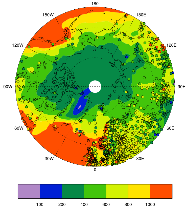
Figure S3. Annual mean precipitation from the ACCMIP 2000 MMM (contours) and observations (filled circles) from Yang et al. (2005).
