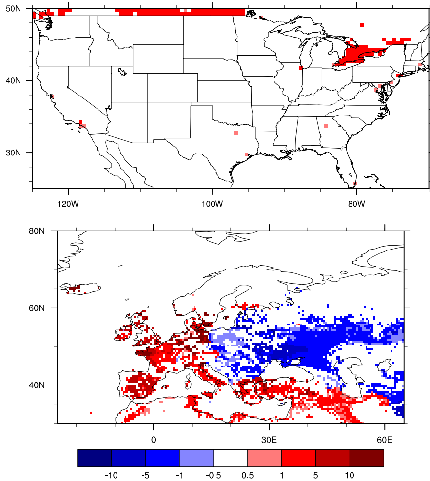
Figure S1b. Change in \text{NH}_3 anthropogenic emissions (2000-1980) in 10^{-2} \text{ mg(N)/m}^2/\text{year} .
