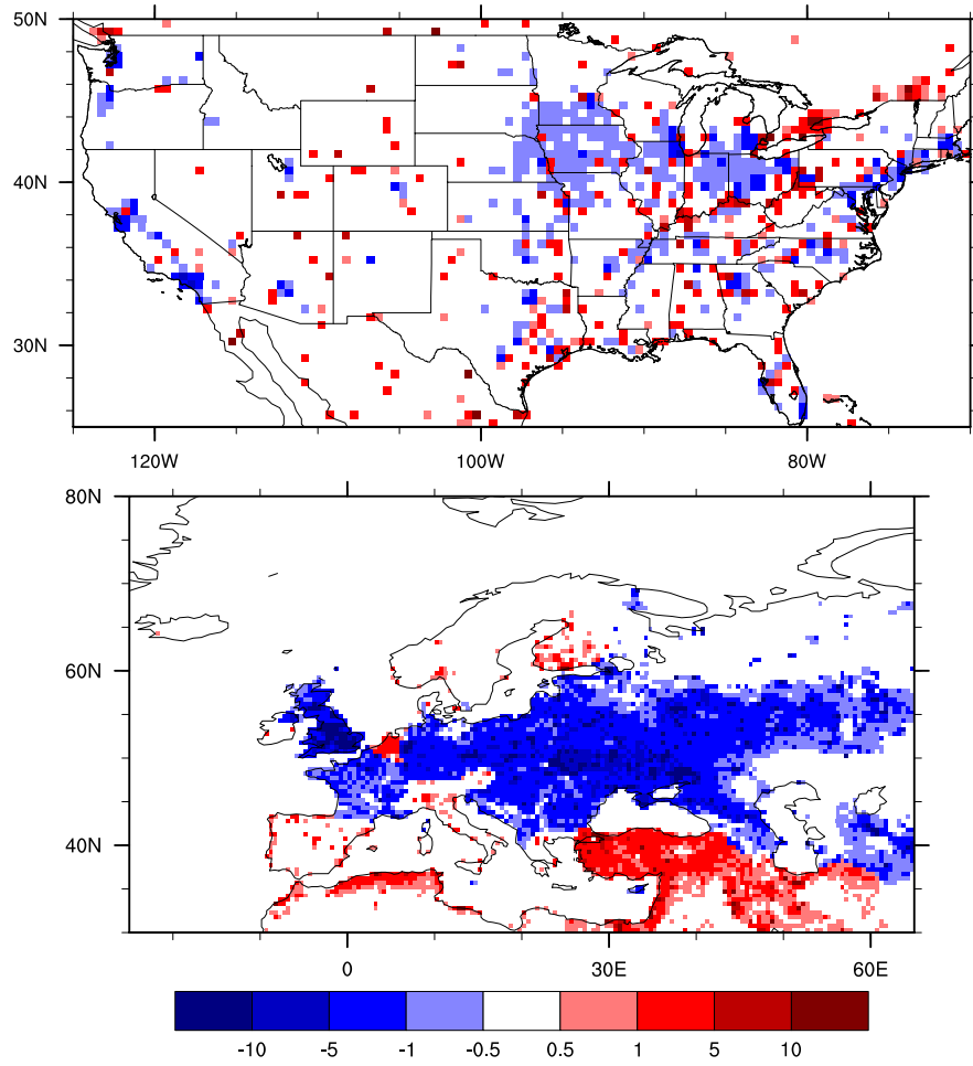
Figure S1a. Change in NO anthropogenic emissions (2000-1980) in 10^{-2} \text{ mg(N)/m}^2/\text{year} .
