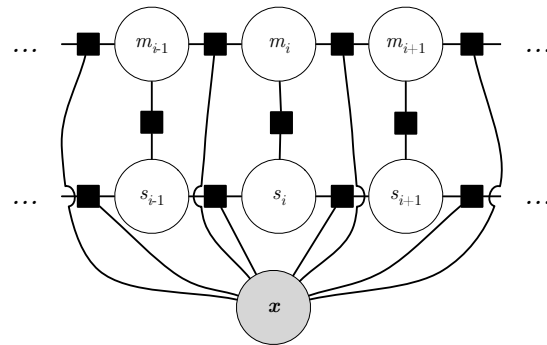
Figure 1: Double-chained CRF expressed as a factor graph: \mathbf{x} is the whole sentence. For a token in position i , its MWE label is m_i and its supersense tag is s_i .
