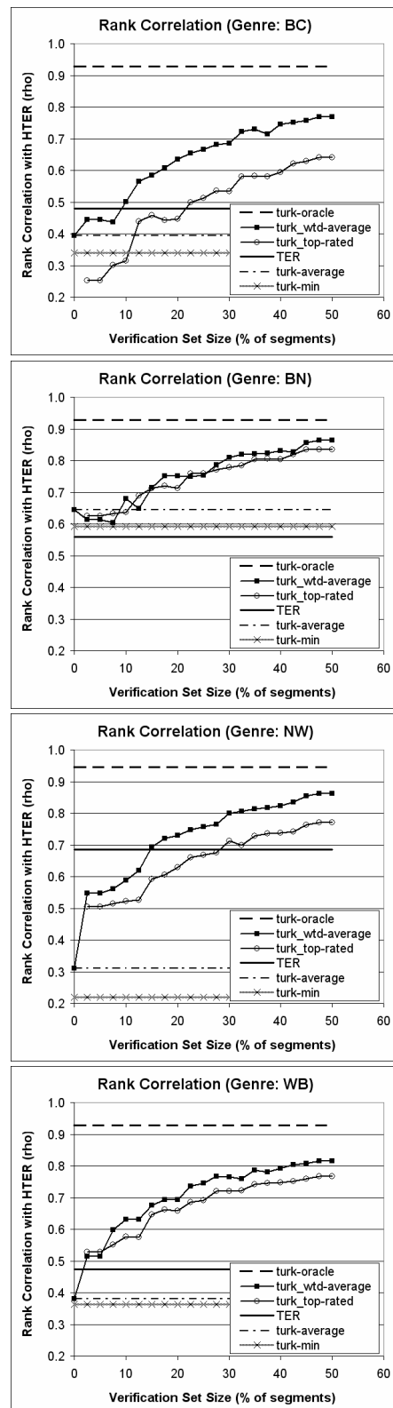
Figure 1: Rank correlation between predicted ranking and HTER ranking for different prediction schemes, across the four genres, and across various sizes of the worker verification set.
