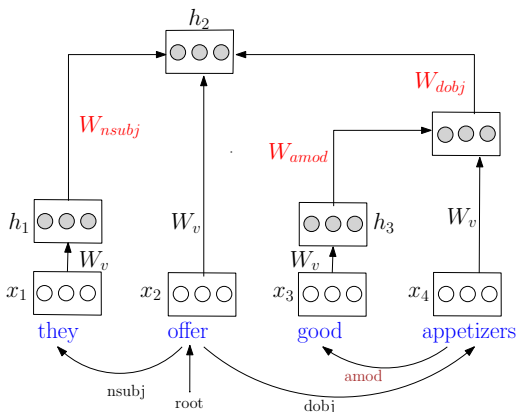
Figure 3 The structure of a dependency-tree-based recursive neural network.
