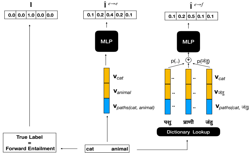
Figure 3: Illustration of weakly supervised training: For a given English example ( cat , animal ), we generate predictions \hat{\mathbf{I}}^{e \rightarrow e} using the monolingual English teacher model. Simultaneously, we also generate predictions \hat{\mathbf{I}}^{e \rightarrow f} using the cross-lingual student model after translating one of the two English words using a dictionary. The cross-lingual classifier attends to all translation candidates and predicts a class based on a weighted average of their features. The loss is defined as \text{CROSS-ENTROPY}(\hat{\mathbf{I}}^{e \rightarrow e}, \mathbf{I}) + \text{CROSS-ENTROPY}(\hat{\mathbf{I}}^{e \rightarrow f}, \mathbf{I}) + \text{KL-DIVERGENCE}(\hat{\mathbf{I}}^{e \rightarrow f}, \hat{\mathbf{I}}^{e \rightarrow e}) .
