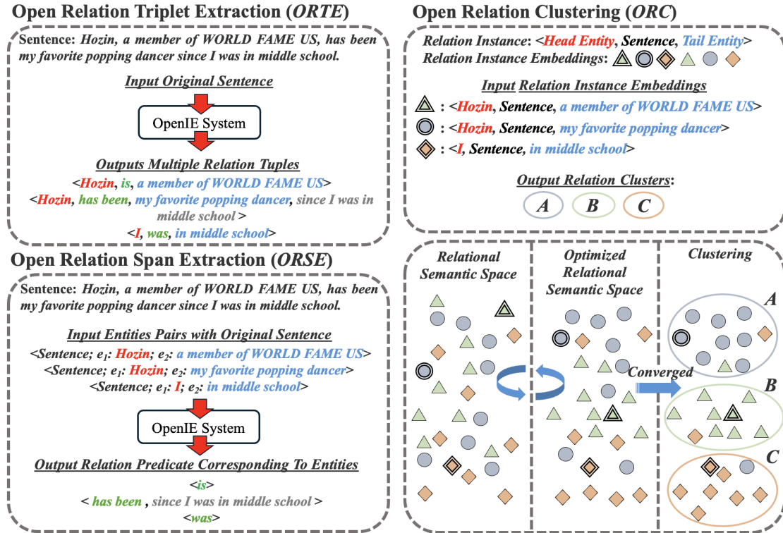
Figure 2: An overview of workflow processes in OpenIE task settings. ORTE aims to extract all n-ary relation tuples in the input, . ORSE finds relational spans according to previously extracted subjects and Objects. ORC pairs the input sentence with different subjects and objects within the sentence to form relation instances, relation instances are iteratively optimized in a supervised, unsupervised, or semi-supervised manner, and after the representations converge, clustering is performed. Objects of the same color indicate that they belong to the same relation cluster. To facilitate observation, we have bolded the borders of the three examples in the figure. Each circle represents the relation instances clustered into the same class by the clustering algorithm.
