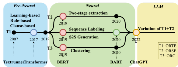
Figure 3: Chronological overview of Open IE methods.
