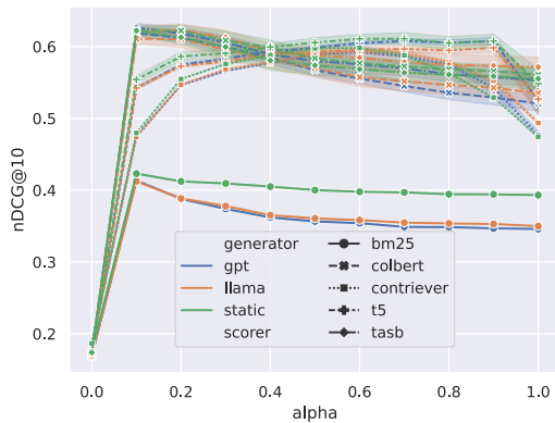
Figure 4: Sensitivity to \alpha measuring nDCG@10 for position absolute 'after'.
