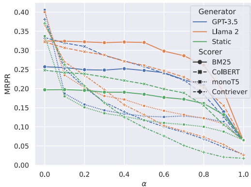
Figure 5: Sensitivity to \alpha measuring nDCG@10 for position absolute 'after'.
