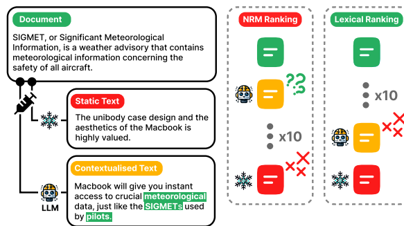
Figure 1: Injection of static and contextualised (document-conditioned by Llama 2) text into a document. BM25 penalises both injections as lexical models estimate relevance in an axiomatic fashion; document length has increased with insufficient additional relevant information. However, the NRM (monoT5) is invariant to the addition of contextualised promotional text. Further examples are enlisted in Appendix D.
