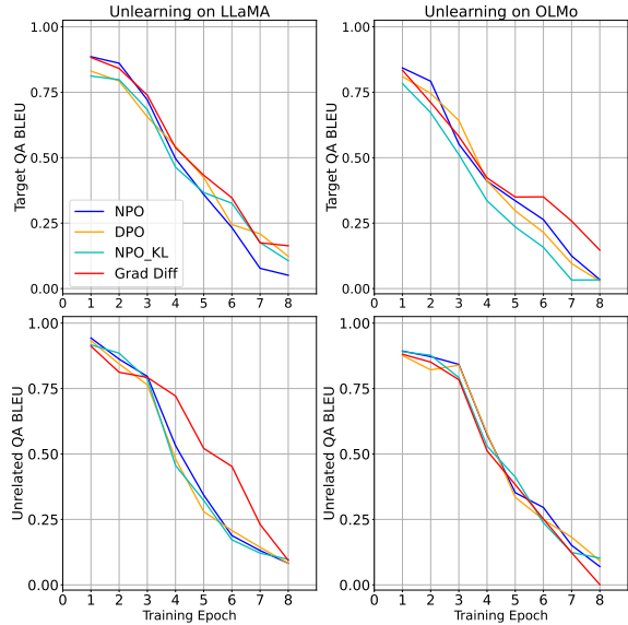
Figure 2: Unlearning testing results on LLaMA and OLMo for each training epoch.
