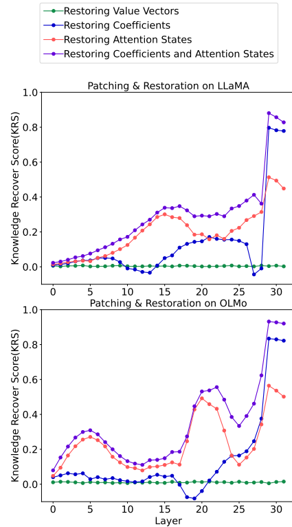
Figure 1: Results of KRS on LLaMA and OLMo under three activations patching or parameters restoration settings. We also included another setting that restores both attention and coefficients to compare the final outcomes.
