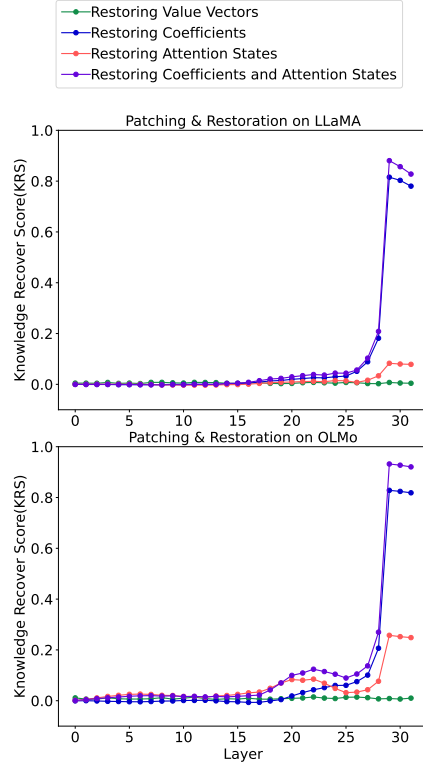
Figure 3: Results of KRS on LLaMA and OLMo under three activations patching or parameters restoration settings, isolating the effects of the two others when investigating each factor individually.
