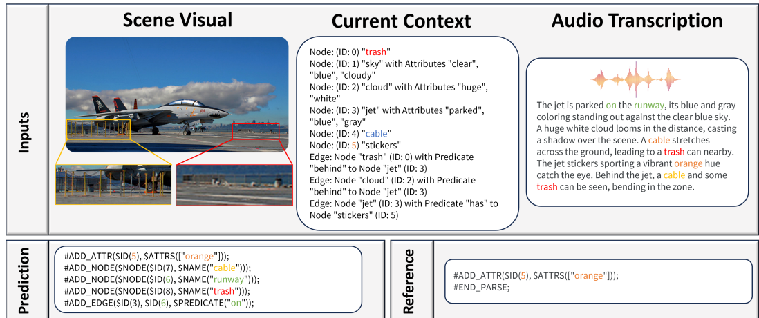
Figure 3: Sample generation output with corresponding inputs from AViD-SP. Scored a Soft-RED of 0.0 and Hard-RED of 6.727. Significant features highlighted in colors. Qualitative evaluation reveals that the majority of extraneous additions were either supported by the Audio Transcription, the scene image, or both.
