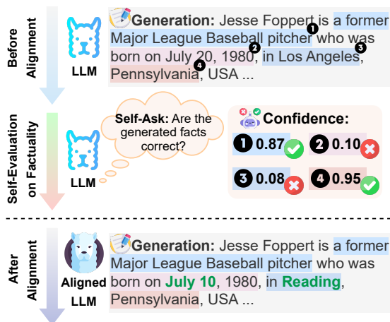
Figure 1: Illustration of Self-Alignment for Factuality . Given a prompt to write a biography, before factuality alignment, the LLM generates some facts that are not accurate. Through self-evaluation, the LLM is capable of identifying these inaccurate facts. The feedback from the self-evaluation is used as a reward signal to align the LLM towards factuality. Each fact is highlighted in distinct colors, and the corrected facts are marked with green letters.
