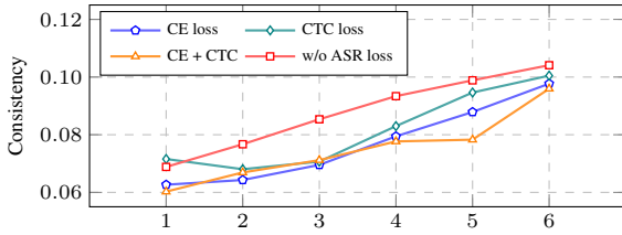
Figure 4: Influence of textual encoder by ASR training strategy.
