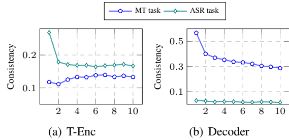
Figure 7: Changes of consistency along training epochs.
