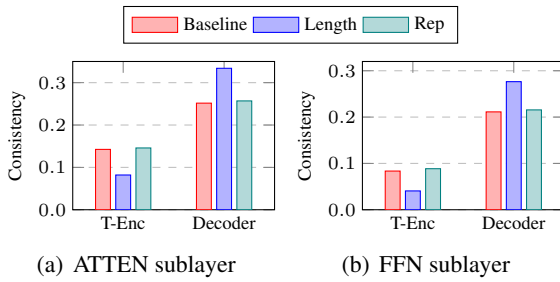
Figure 5: Consistency of different modules.
