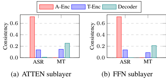
Figure 2: Consistency of different tasks in different modules.
