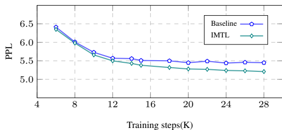
Figure 11: PPL of Dev set during training.
