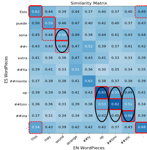
Figure 2: We compute a pair-wise cosine similarity matrix to simulate word alignments. For each column, we look only at source word-pieces with an associated label and keep the top-k (k=2) most similar target-side word piece candidates (red squares). The black circles show the aligned full-word.
