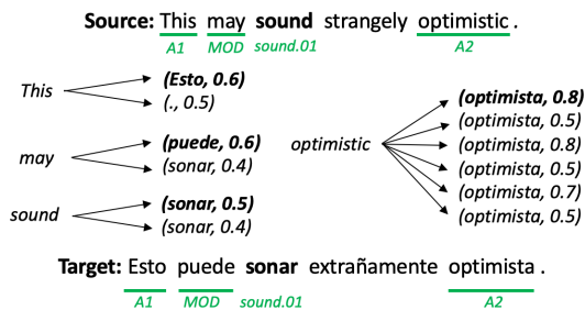
Figure 3: We map word pieces to full-words and apply filters to obtain final source-to-target word alignments.
