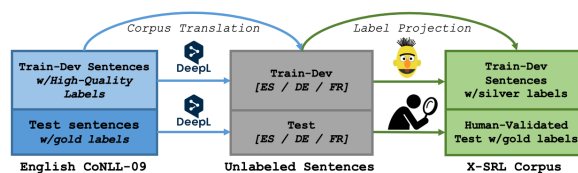
Figure 1: Method to create X-SRL. We automatically translate the English CoNLL-09 corpus, use a fast label projection method for train-dev and get human annotators to select the appropriate head words on the target sentences to obtain gold annotations for the test sets.
