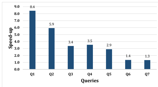
Figure 12: Query Latency Speedup
