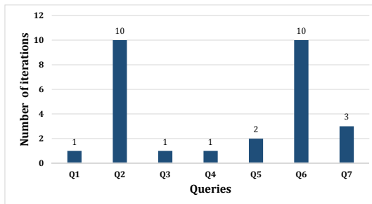
Figure 13: Number of Iterations before Convergence
