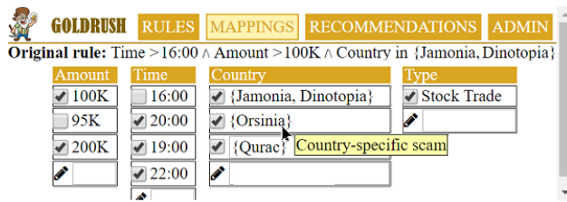
Figure 5: GOLDRUSH UI: Mappings (concretization)
