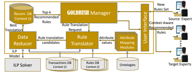
Figure 4: GOLDRUSH architecture
