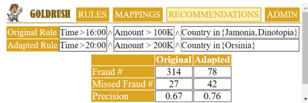
Figure 6: GOLDRUSH UI: Recommended Translations
