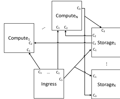
Figure 11: Network Flow Diagram for Active-Active Periodic Checkpointing
