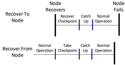
Figure 4: On Demand Checkpointing Based Timeline
