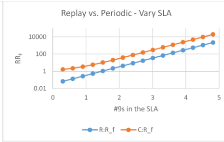
Figure 17: Replay vs. Periodic - Vary SLA, Measure RR_F
