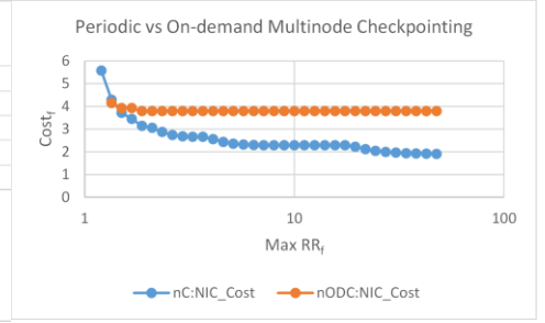
Figure 21: Periodic vs On-Demand Checkpointing - Vary RR_F
