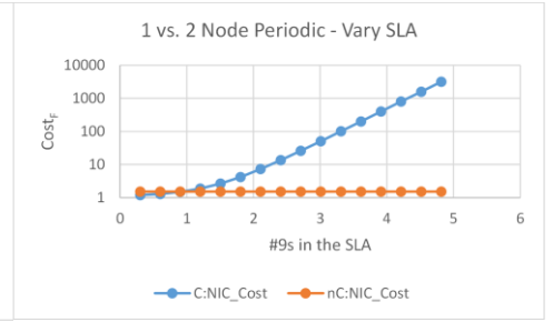
Figure 18: 1 vs. 2 Node Periodic - Vary SLA, Measure Cost_F
