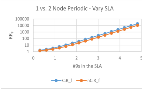
Figure 19: 1 vs. 2 Node Periodic - Vary SLA, Measure RR_F
