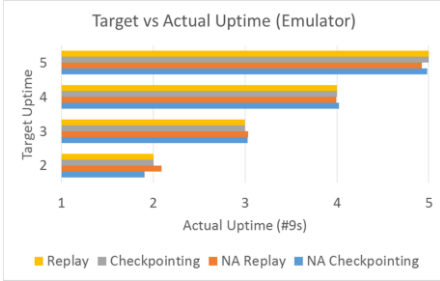
Figure 13: Target vs Actual Uptime
