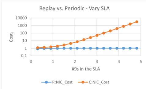
Figure 16: Replay vs. Periodic - Vary SLA, Measure Cost_F
