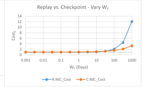
Figure 15: Replay vs. Checkpoint - Vary W_T
