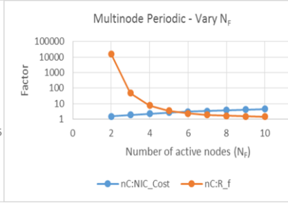
Figure 20: Multinode Periodic - Vary N_F , Measure Cost_F & RR_F
