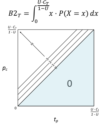
Figure 10: Case 2 variables and integration limits
