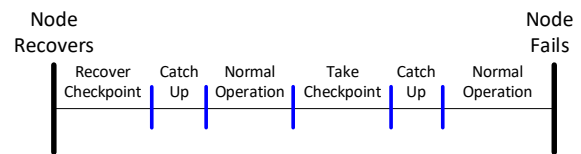
Figure 3: Periodic Checkpointing Based Timeline
