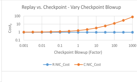
Figure 14: Replay vs. Checkpoint - Vary Checkpoint Blowup
