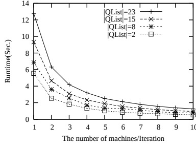
Figure 8: Scalability in query size
