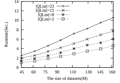
Figure 12: Scalability in data
