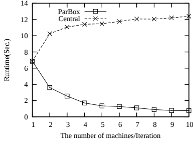
Figure 7: ParBoX vs. NaiveCentralized
