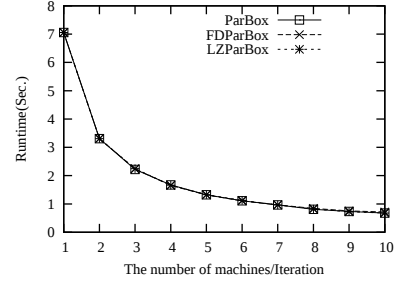
Figure 9: Query q_{F_0}
