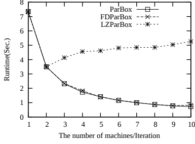
Figure 10: Query q_{F_n}
