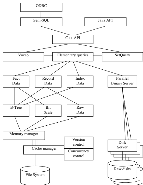
Figure 2. Sem-ODB Engine architecture
