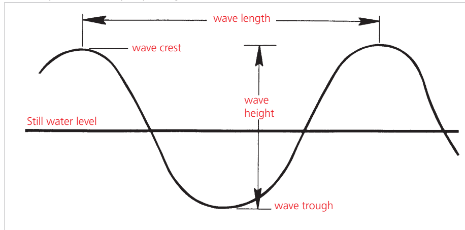
Figure 18 Characteristics of a wave.
