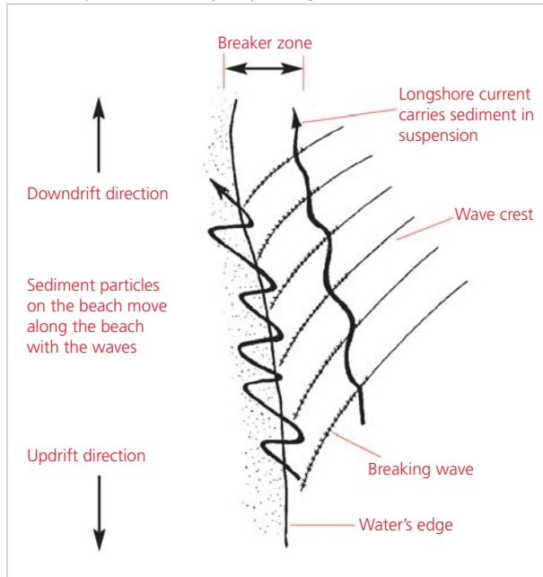
Figure 21 Longshore currents.
