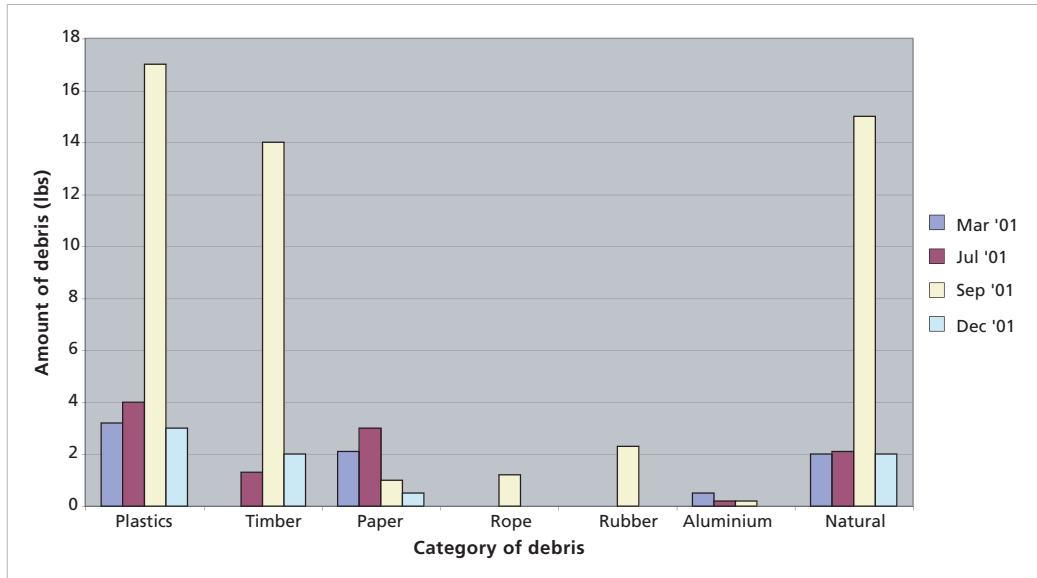
Figure 15 Bar graph showing beach debris changes.
