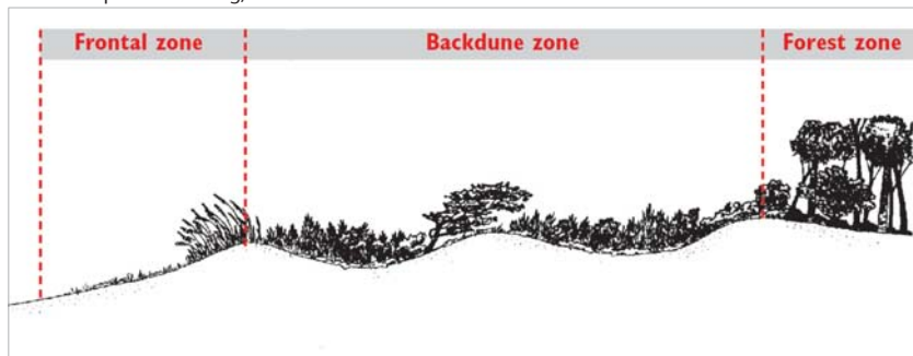
Figure 26 Vegetation succession: the frontal zone is covered with grasses and vines, which gives way to shrubs and herbaceous plants and eventually the coastal woodland.
