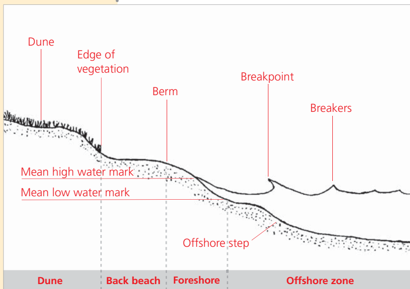
Figure 1 Cross-section of a typical beach.
