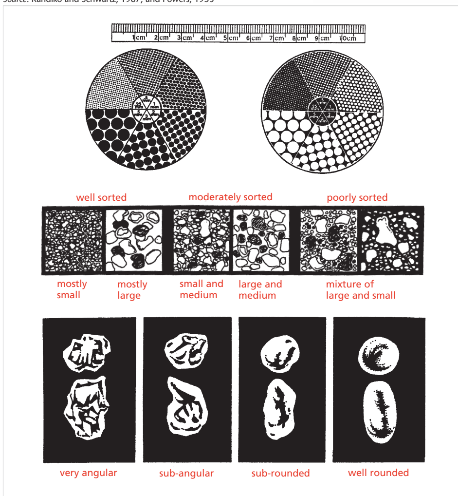
Figure 11 Sediment analysis charts for size, shape and sorting.
