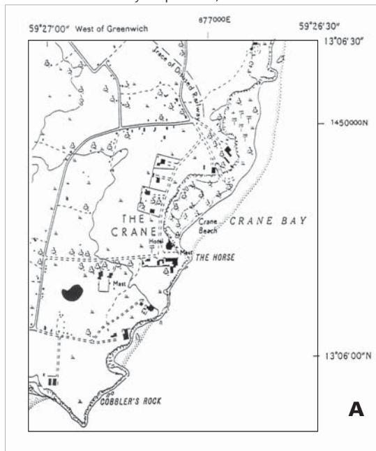
Figure 4 Different perspectives of Crane Beach, Barbados. (A – topographic map from 1970s, B – aerial photograph from 1970s, C – aerial photograph from Google Earth from 2006, and D – ordinary photograph from 1970s).
