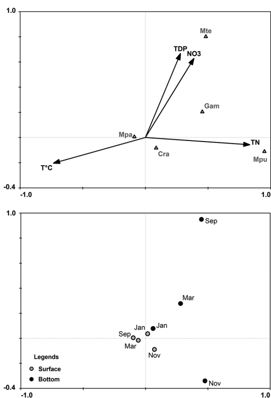
Figure 2. Canonical correlation analysis (CCA) biplot showing the relationship between the abundant phytoplankton species and abiotic conditions of Mundaú reservoir, Pernambuco, Brazil. Note: Jan = January, Mar = March, Sep = September, and Nov = November; the symbols represent water column depths, i.e. subsurface and bottom. NO 3 = nitrate; TDP = total dissolved phosphorus; TN = total nitrogen; T°C = water temperature; Cra = Cylindrospermopsis raciborskii ; Gam = Geitlerinema amphibium ; Mpa = Microcystis panniformis ; Mpu = Merismopedia punctata and Mte = Merismopedia tenuissima .
