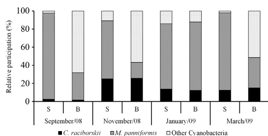
Figure 1. Biomass variation of total cyanobacterial population, C. raciborskii , M. panniformis and other cyanobacteria without C. raciborskii and M. panniformis in the subsurface (S) and at the bottom (B) of the water column of Mundaú reservoir, Pernambuco, Brazil.
