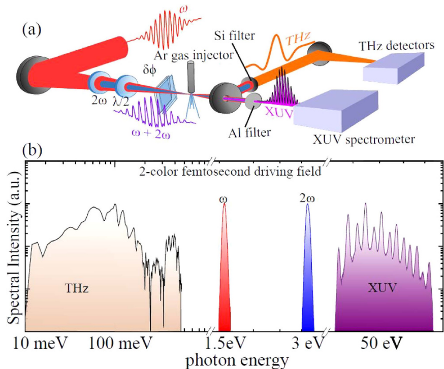
Figure 1. Coherent ultrabroadband emission from 2-color optical pulses focused into an argon gas jet.
