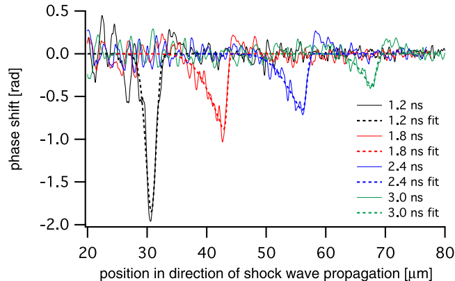
Figure 3. Phase profiles of the shock front at different time delays.
