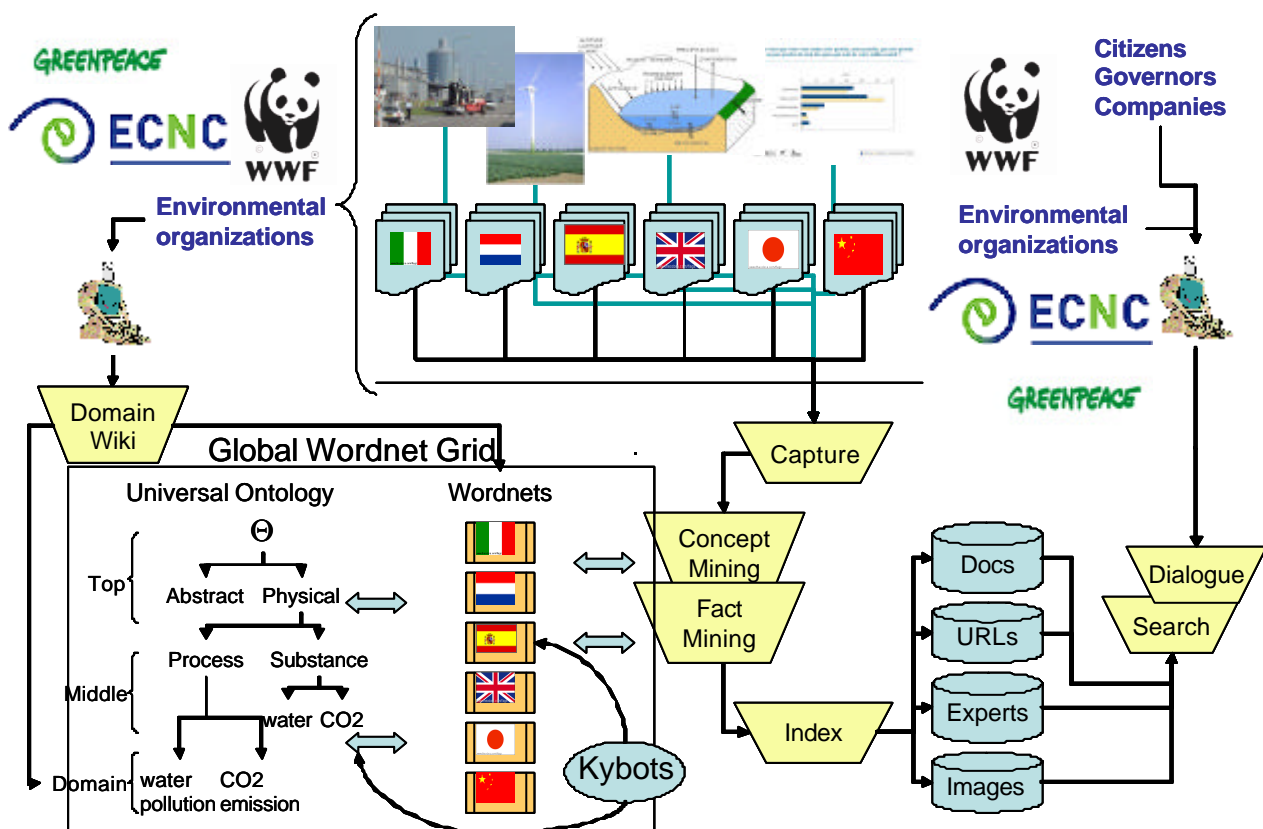
Figure 1: System architecture
