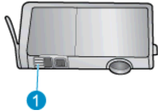
1 Electrical contacts
