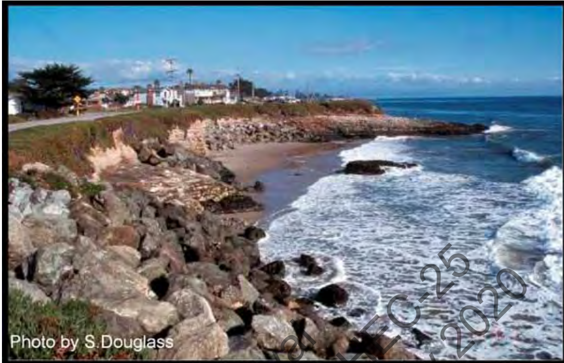
Figure 6.11. Seawall protecting a local road. West Cliff Drive, Santa Cruz, California
