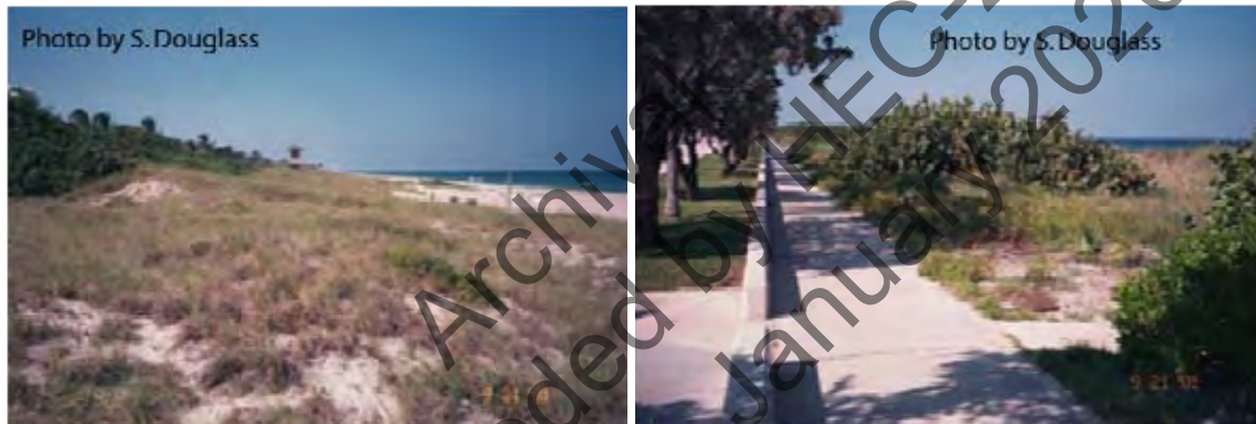
Figure 7.16. Beach nourishment project with constructed dune on top of old, failed revetment protecting road. Florida Highway A1A, Delray Beach (2001)
