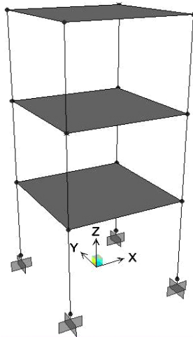
Fig. 3: Steel Frame
