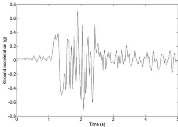
Fig. 4: The Naghan earthquake records (Iran 1977)
