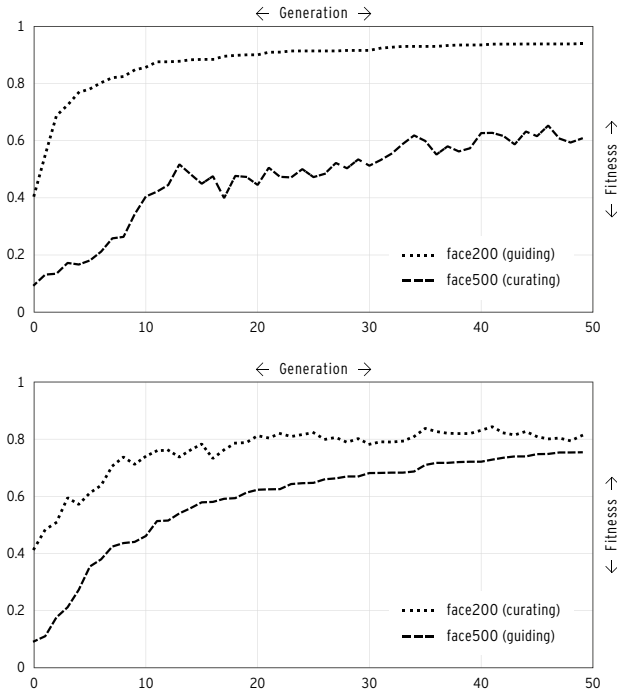
Figure 5: Evolution of the fitness of the best individual throughout generations when using face200 to guide evolution and face500 to curate individuals (top); and the other way around (bottom). The visualised results are averages of 30 runs.
