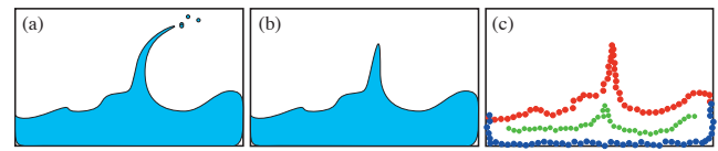
Figure 3: (a) The liquid shape at the selected frame contains tiny splashes. (b) These splashes are discarded by extracting the main body of liquid. (c) Three fluid particle subsets are extracted (red for free surface particles, blue for solid boundary particles and green for medial axis particles).
