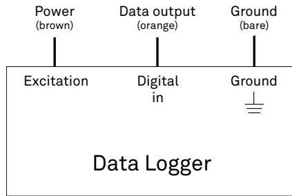
Figure 4 Wiring diagram
