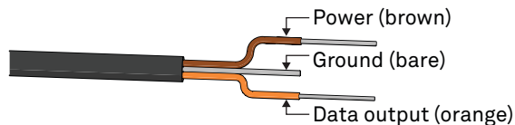
Figure 3 Pigtail wiring
