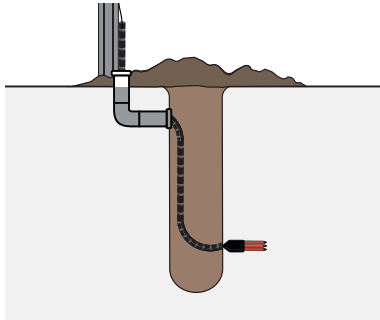
Figure 1 Example of 5TM proper installation
