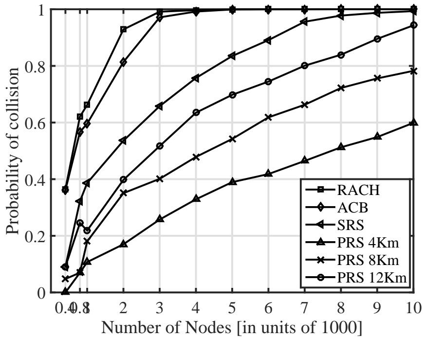
Figure 4.8: Collision probability of representative RA schemes in homogeneous network
