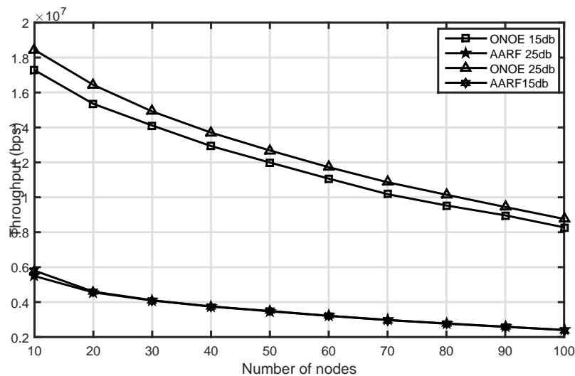
Figure 6.3: Performance of legacy algorithms in static network with SNR of 15db
