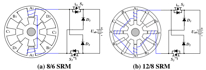
(a) 8/6 SRM (b) 12/8 SRM Fig. 1. Basic winding structure of SRM.
