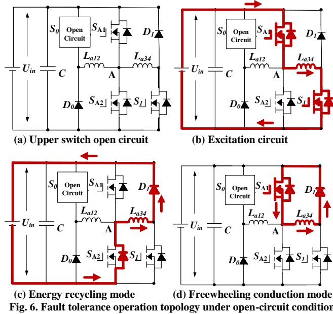
Fig. 6. Fault tolerance operation topology under open-circuit condition.
