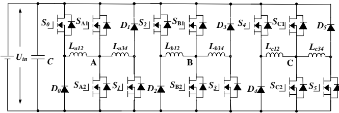
(a) Proposed fault tolerance topology
