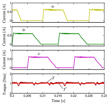
Fig. 19. Simulation results of current regulation control mode with fault tolerance topology under fault conditions.
