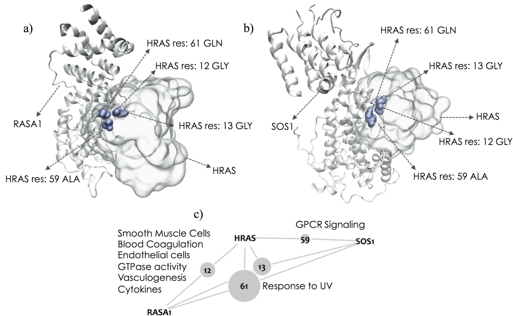
Figure3. The RASA1–HRAS complex (a) and the SOS1–HRAS complex (b) show that both interactors utilize the same binding site on HRAS. Residues 12, 13, 59 and 61 on HRAS that participate in the interface region of these interactions are highlighted in blue. Residue 12 mediates the HRAS-RASA1, residue 59 mediates the HRAS-SOS1 interaction, and 13 and 61 participate in both interactions. The small network (c) provides a schematic of the residues mediating particular interactions. The grey nodes represent the residues. Their sizes are proportional to the frequency with which they are mutated in the TCGA cohort. Functions predicted to be specifically altered by mutations at each interface are listed on the edges.
