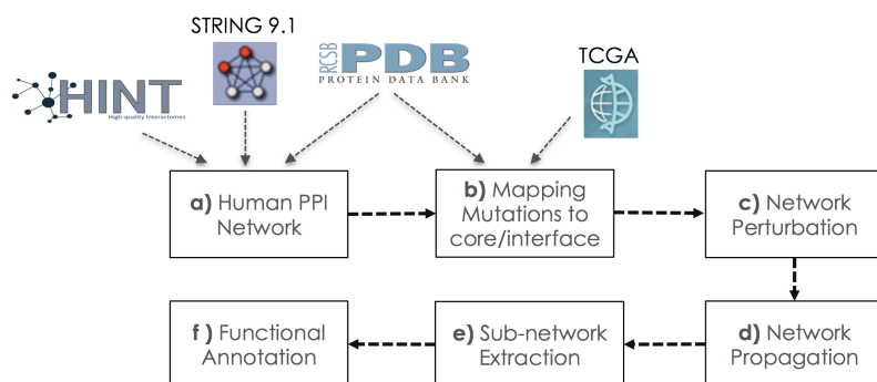
Figure 1. A pipeline for mining molecular cancer related sub-networks accounting for different effects of distinct mutations. Steps include network assembly (a), mapping of mutations to interface versus core residues of cancer genes (b), removal of affected edges (c), extraction of associated protein sets (d & e) and functional annotation (f).
