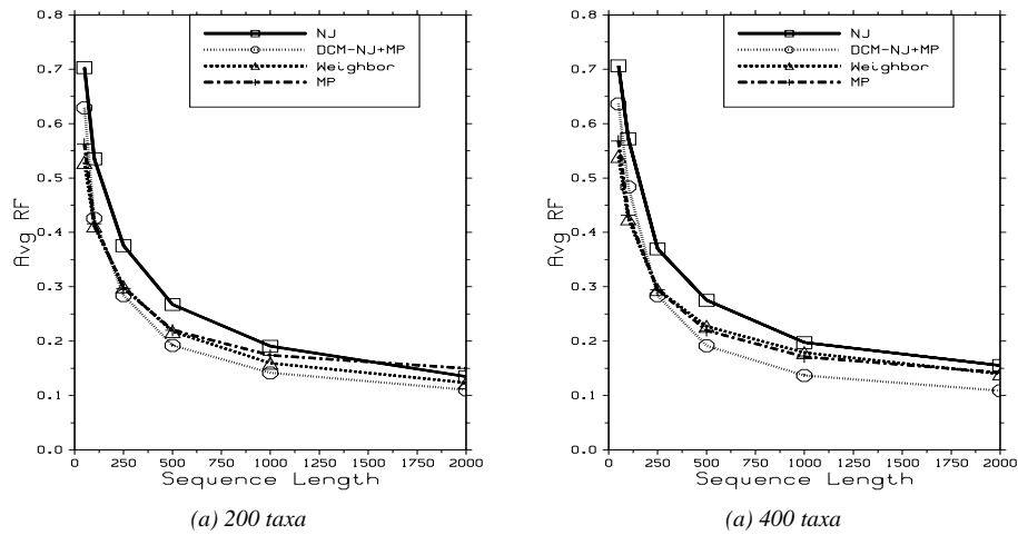
Figure 4: Accuracy as a function of the sequence length under the K2P+Gamma model for expected diameter (2.0) and two numbers of taxa
