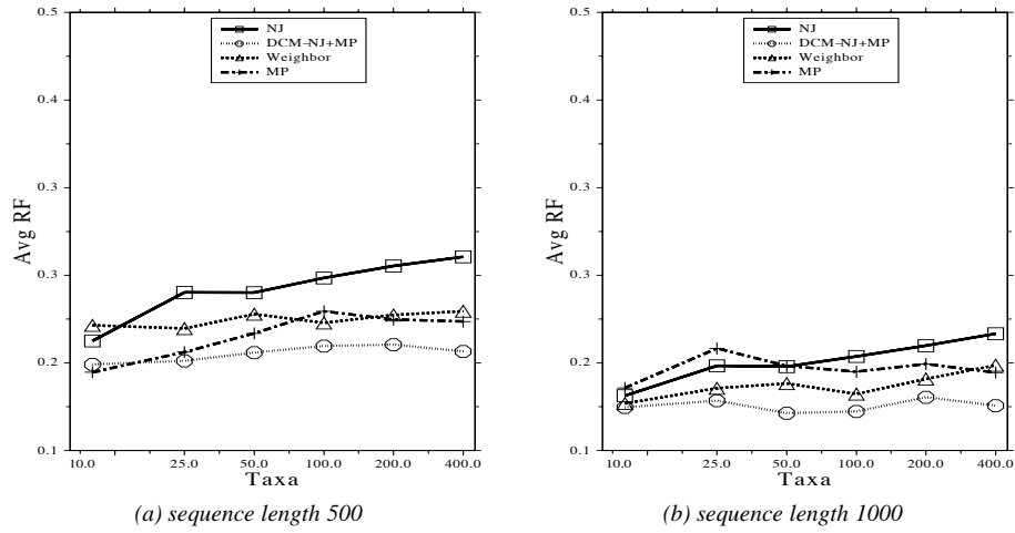
Figure 3: Accuracy as a function of the number of taxa under the K2P+Gamma model for expected diameter (2.0) and two sequence lengths
