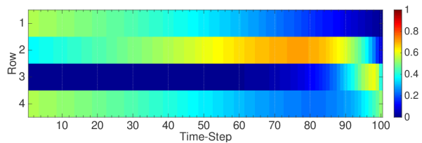
Figure 3. We visualize the power of taking linear combinations of \mu^{(\alpha)} 's for providing different viewpoints into past data. In row 1 we show the effective weights that would be used for weighing statistics \varphi_t if one considers .001^{-1}\mu^{(.999)} - .01^{-1}\mu^{(.99)} ; we see that this is equivalent to considering only statistics from the distant past. Similarly, we show the effective weights when taking .01^{-1}\mu^{(.99)} - .1^{-1}\mu^{(.9)} and .1^{-1}\mu^{(.9)} - .5^{-1}\mu^{(.5)} on rows 2 and 3 respectively. We see that these linear combinations amount to considering viewpoints concentrated at various points in the past. Lastly its worth noting that more complicated linear combinations may lead to even richer views on previous statistics; for instance, we show .001^{-1}\mu^{(.999)} - .01^{-1}\mu^{(.99)} + .5^{-1}\mu^{(.9)} on row 4, which concentrates on the statistics of the distant and very recent past, but de-emphasizes statistics of data from less recent past.
