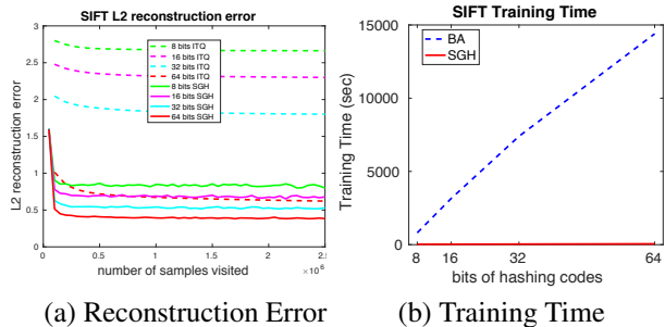
Figure 1: (a) Convergence of reconstruction error with number of samples seen by SGD, and (b) training time comparison of BA and SGH on SIFT-1M over the course of training with varying number of bits.
