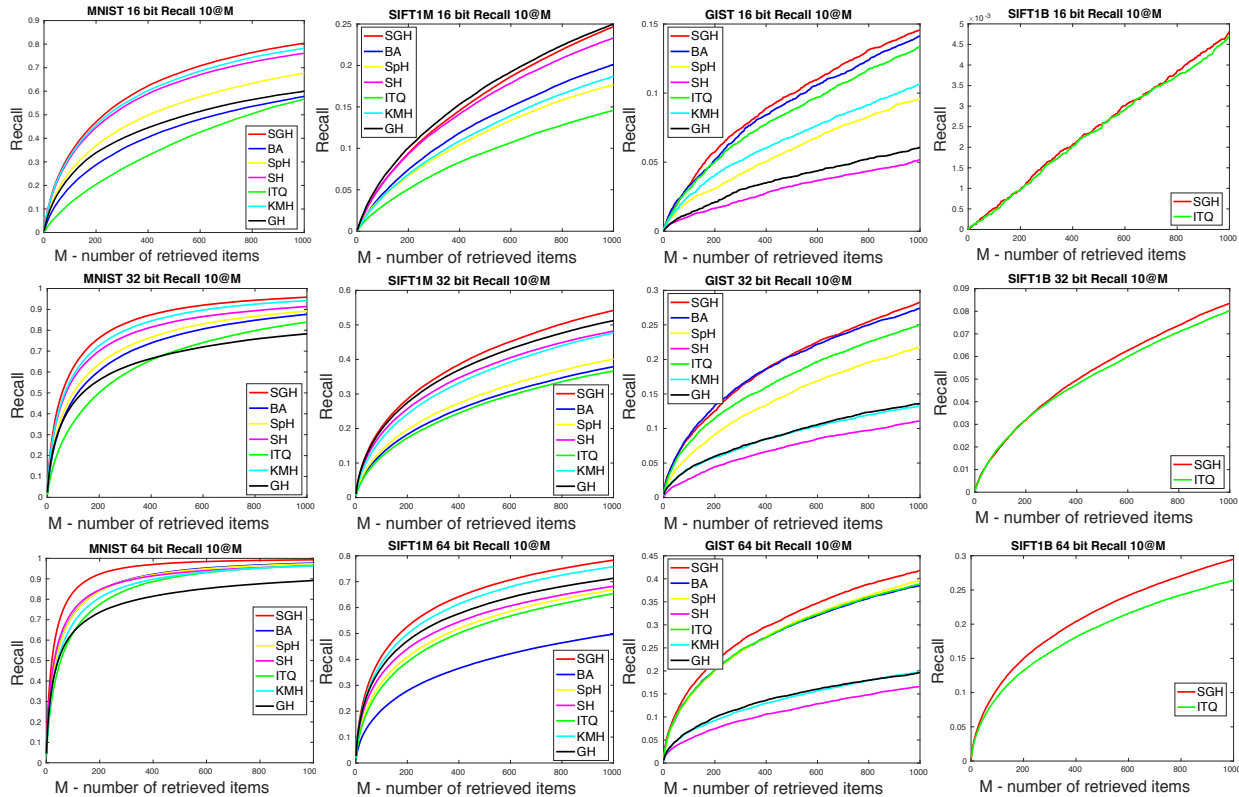
Figure 2: L2NNS comparison on MNIST, SIFT-1M, and GIST-1M and SIFT-1B with the length of binary codes varying from 16 to 64 bits. We evaluate the performance with Recall 10@ M (fraction of top 10 ground truth neighbors in retrieved M ), where M increases up to 1000.
