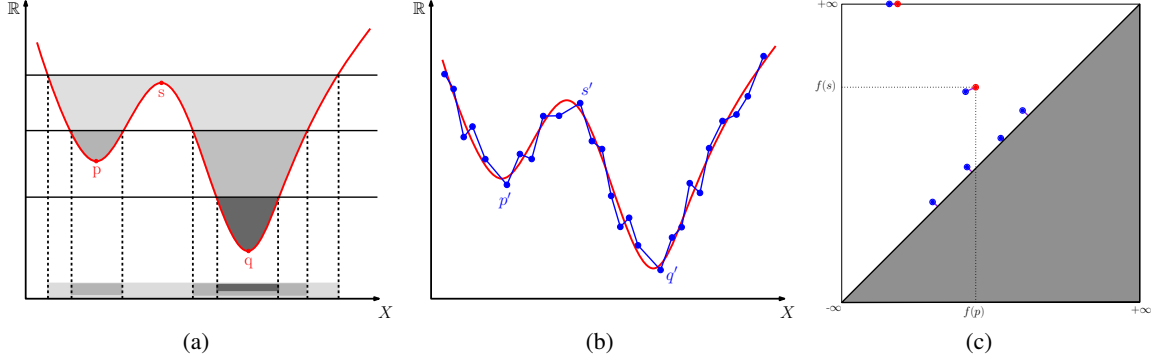
Figure 1. Sketch of persistent homology: (a) the horizontal lines are the boundaries of sublevel sets f^{-1}((-\infty, t]) , which are colored in decreasing shades of grey. The vertical dotted lines are the boundaries of their different connected components. For instance, a new connected component is created in the sublevel set f^{-1}((-\infty, t]) when t = f(p) , and it is merged (destroyed) when t = f(s) ; its lifespan is represented by a copy of the point with coordinates (f(p), f(s)) in the persistence diagram of f (Figure (c)); (b) a piecewise-linear approximation g (blue) of the function f (red) from sampled values; (c) superposition of Dg f (red) and Dg g (blue), showing the partial matching of minimum cost (magenta) between the two persistence diagrams.
