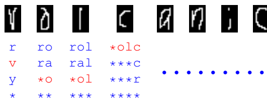
Figure 1. In handwriting recognition, we want to output a letter at each position. Our model also chooses a context at each position that summarizes the outputs so far (e.g., *olc remembers only the last three letters) and is used for predicting the next letter. By selecting contexts at multiple levels of resolution, our model can place probability mass over the entire output space while still capturing complex dependencies.
