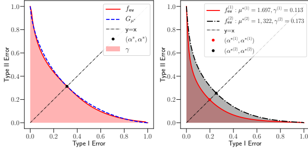
Figure 4.1. Left: An illustration of the (\mu^*, \gamma) parameterization. Right: f_{EW}^{(2)} is more private than f_{EW}^{(1)} .
