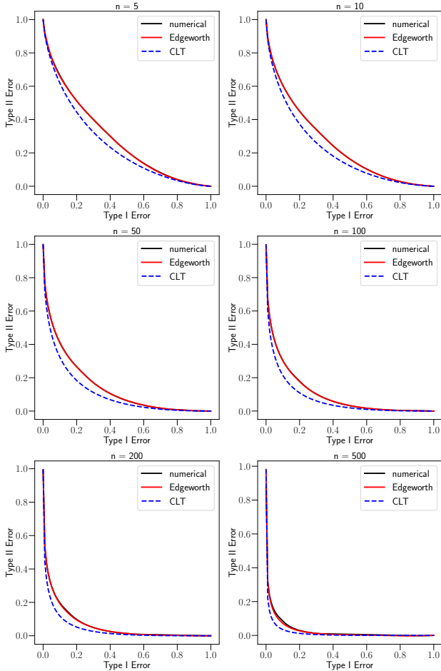
Figure 5.4. The estimation of the privacy bound for n -step noisy SGD. The sampling rate is p = 0.5/n^{1/4} and the noise scale is \sigma = 1 .
