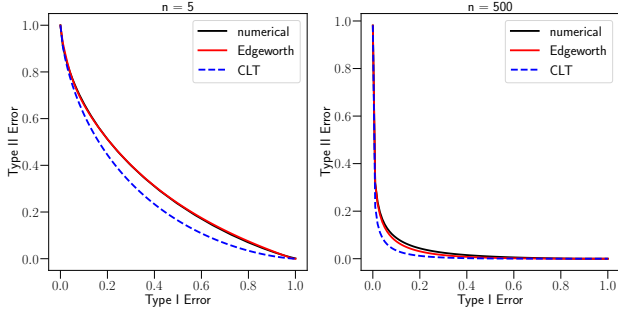
Figure 5.3. The estimation of 0.5/n^{1/4}(G_1 + \text{Id})^{\otimes n} .
