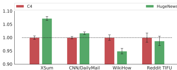
Figure 3: Effect of pre-training corpus. PEGASUS BASE pre-trained on C4 (350M Web-pages) and HugeNews (1.5B news-like documents).
