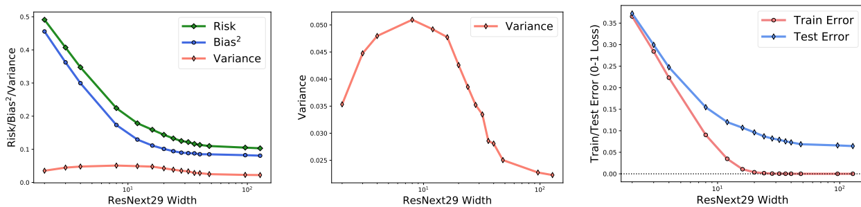
Figure 7. Risk, bias, variance, train/test error for ResNext29 trained by MSE loss on CIFAR10 dataset (25,000 training samples). (Left) Risk, bias, and variance for ResNext29. (Middle) Variance for ResNext29. (Right) Train error and test error for ResNext29.
