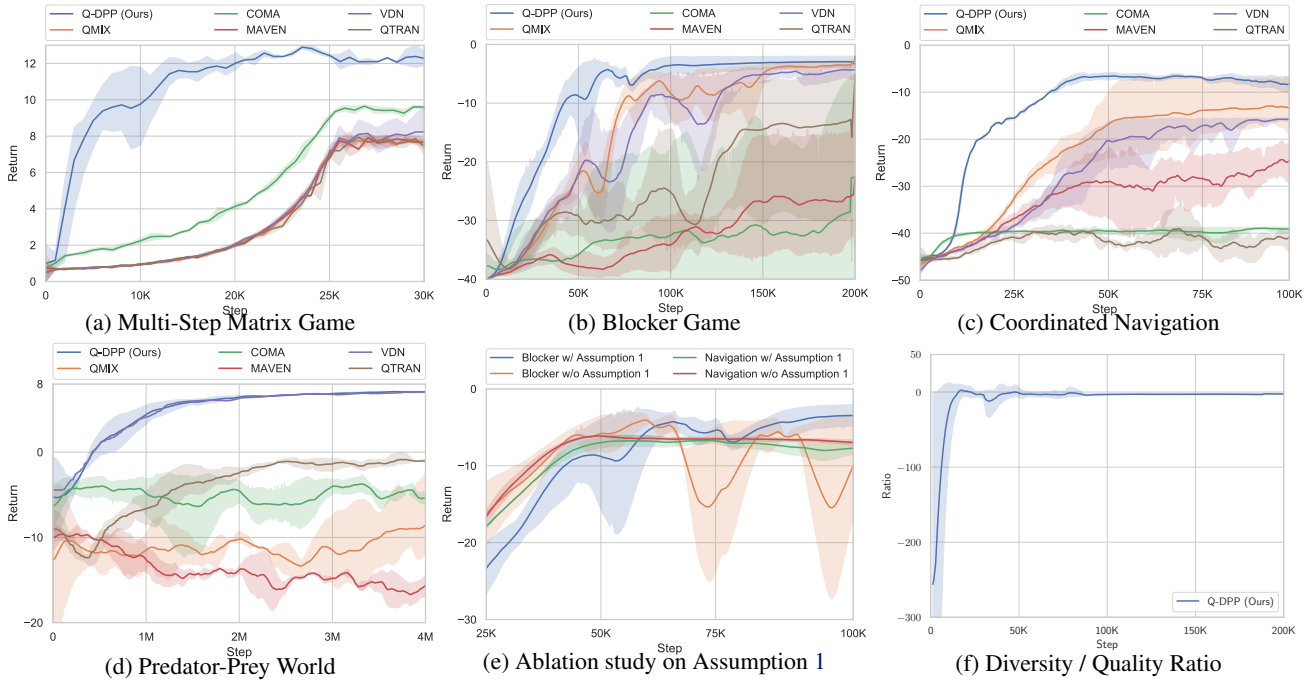
Figure 4: (a)-(d) : Performance over time on different tasks. (e) : Ablation study on Assumption 1 on Blocker game. (f) : The ratio of diversity to quality, i.e., \log \det(\mathcal{B}_Y^T \mathcal{B}_Y) / \sum_{i=1}^N Q_{\mathcal{I}(o_i, a_i)}(o_i, a_i) , during training on Blocker game.
