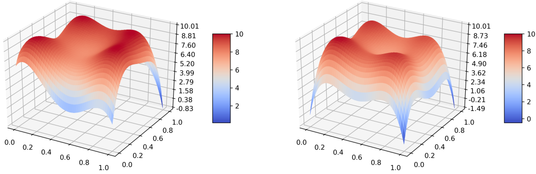
Figure 4. Landscapes of test functions used in Section 7. Left : (Rescaled) Himmelblau's function. Right : (Rescaled) Styblinski-Tang function.
