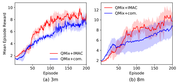
Figure 6. Learning curves comparing IMAC to other methods for 3m and 8m in Starcraft II.
