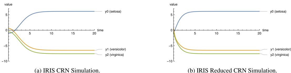
Figure 2. Simulation of IRIS CRN (left) and IRIS CRN in reduced form (right) on the same example. Plots show concentrations of the output species over time, i.e., the difference between positive and negative output species ( y_i(t) = y_i^+(t) - y_i^-(t) ). Networks classify given input with label 0. The reduced CRN converges significantly faster. Note that the initial concentrations of output species change after optimization based on the biases in the ReLU network, as described in Section 3.3.
