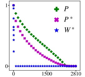
Figure 2. Portion of absolute eigenvalues (sorted and rescaled) for CORA-ML with CELL trained to 50% edge overlap for H = 9 .
