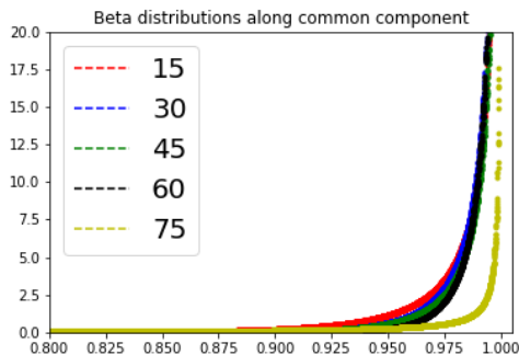
(a) Beta fit on estimated probabilities of correct class using common common component.
