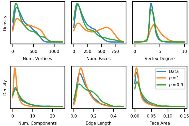
Figure 7. Distribution of mesh statistics for unconditional samples from our model and the ShapeNet test set. We compare samples generated with nucleus sampling and top- p = 0.9 , to true model samples.
