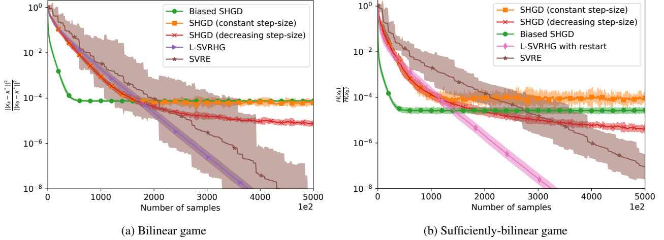
Figure 3. Results for the bilinear game and sufficiently-bilinear game with symmetric positive definite matrices. We observe results very similar to the results observed in section 7.1 and section 7.2, the experiments again shows that our proposed methods follow closely the theory and that L-SVRHG is the fastest method to converge.
