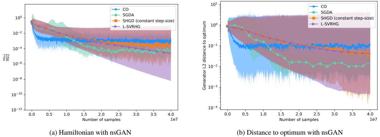
Figure 5. nsGAN with batch size of 100
